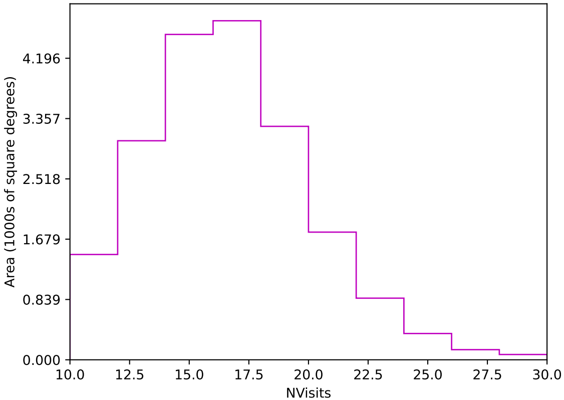
internal_u_expt38_nscale1.2v3.4_10yrs Yr 1 z band: NVisits
