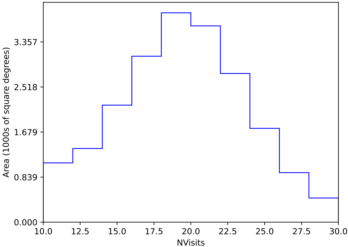
internal_u_expt38_nscale1.2v3.4_10yrs Yr 1 y band: NVisits
