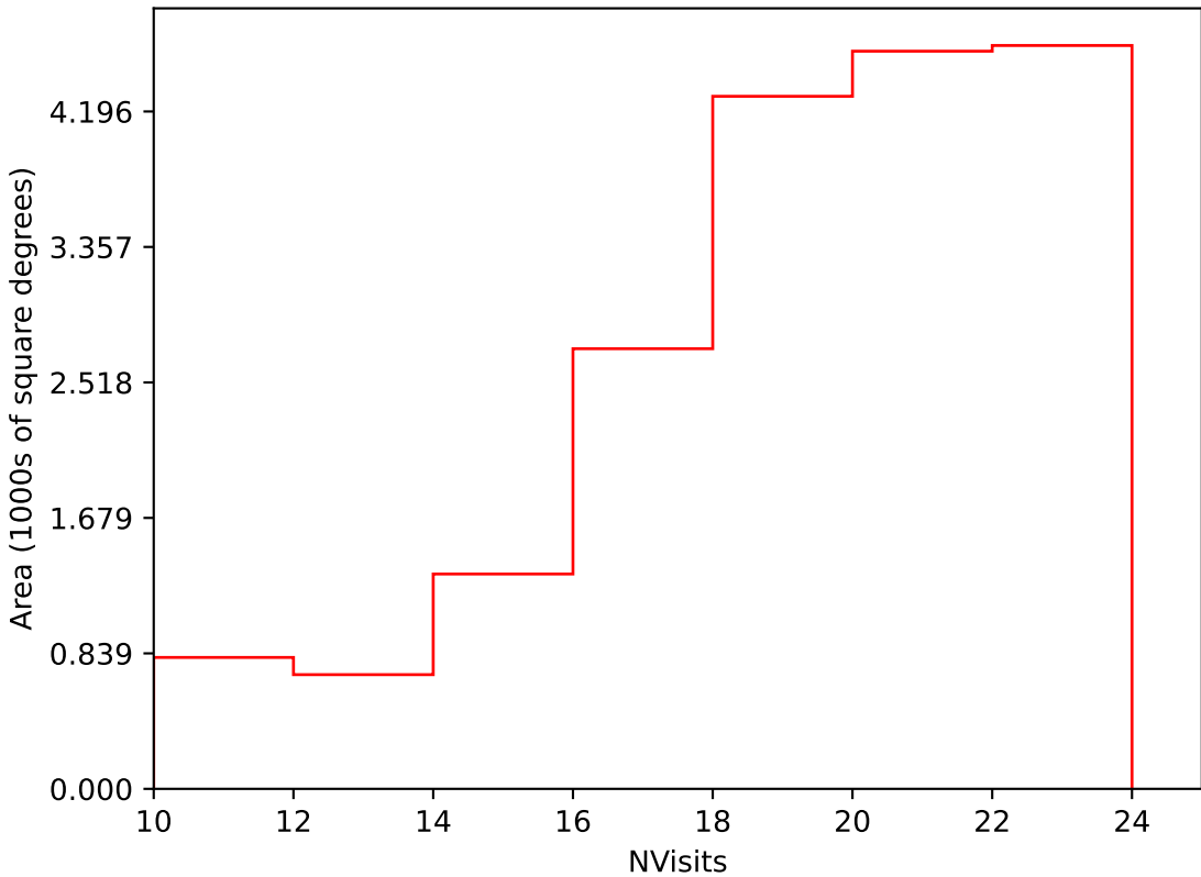
internal_u_expt38_nscale1.2v3.4_10yrs Yr 1 i band: NVisits
