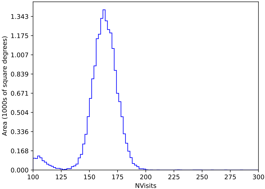
internal_u_expt38_nscale1.2v3.4_10yrs WFD y band: NVisits
