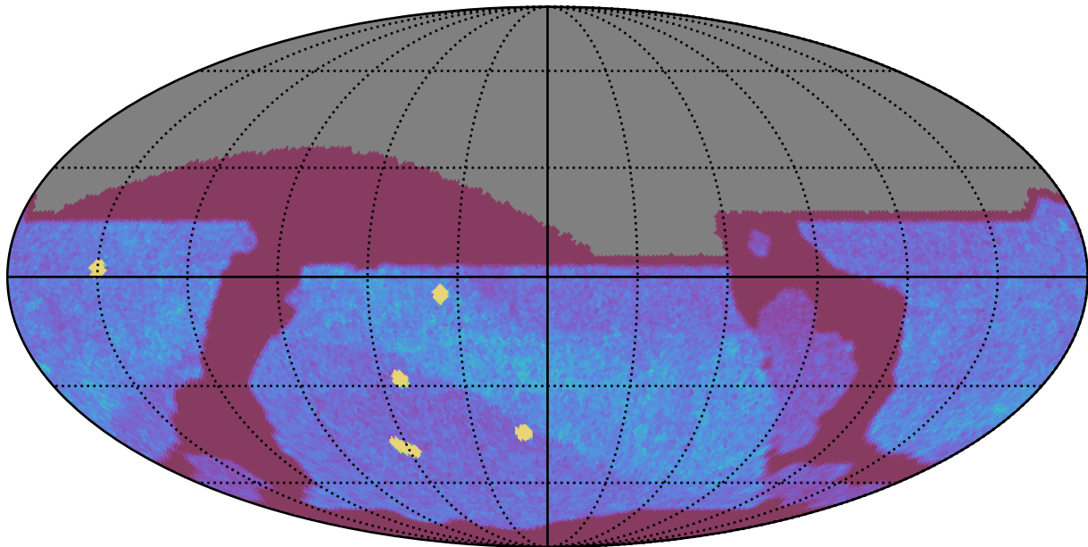
internal_u_expt38_nscale1.2v3.4_10yrs All sky z band: NVisits
