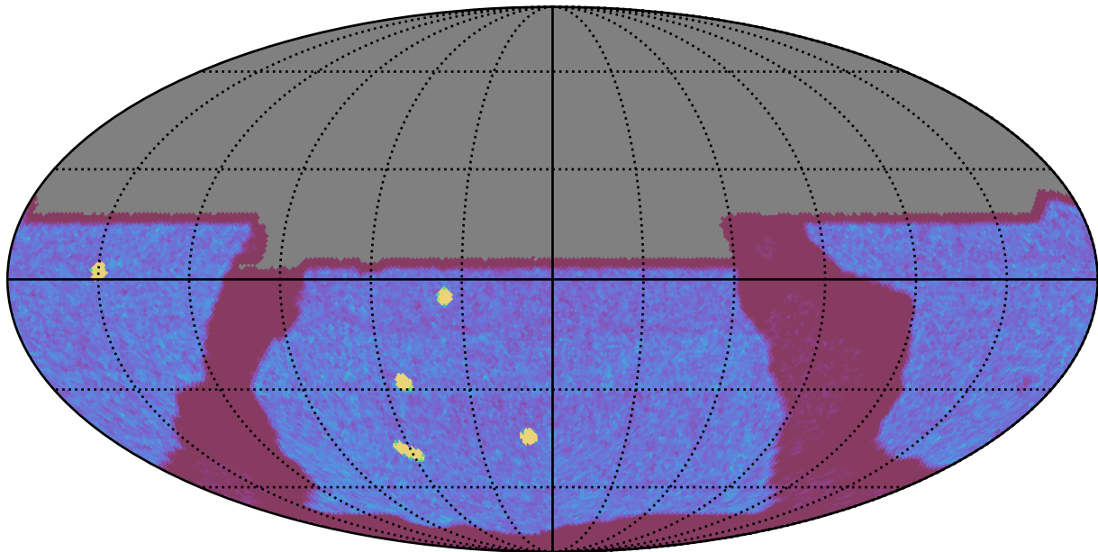
internal_u_expt38_nscale1.2v3.4_10yrs All sky y band: NVisits
