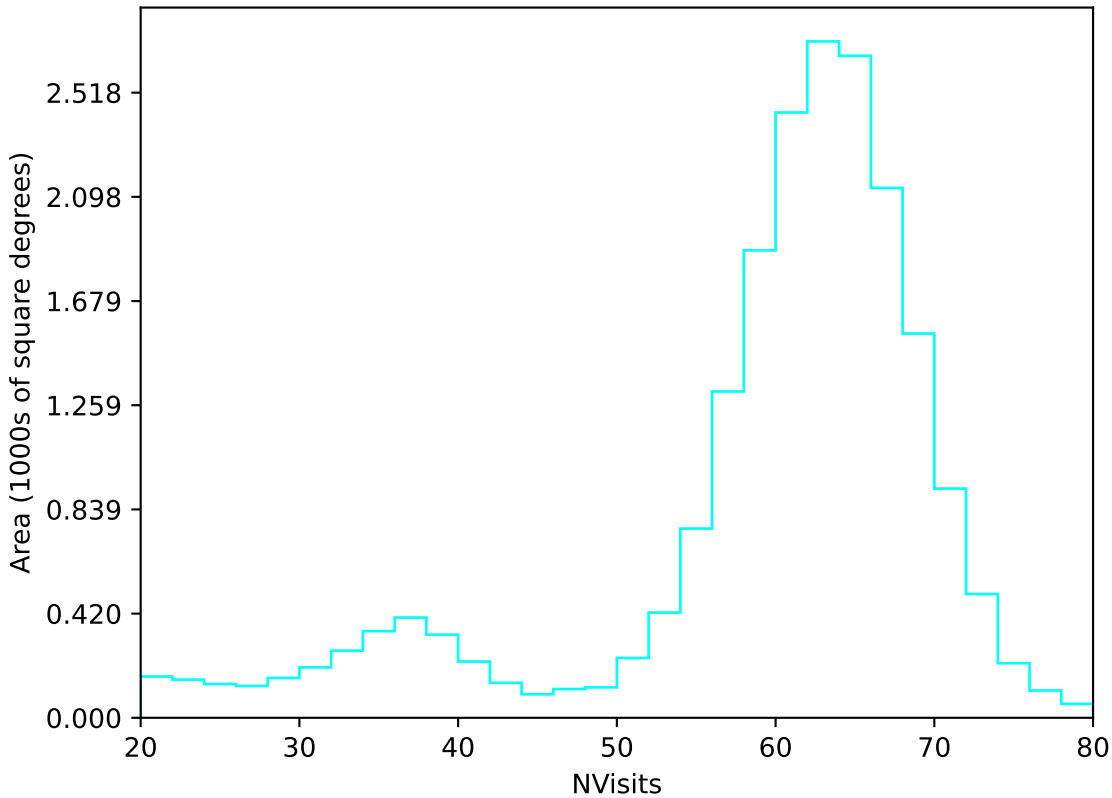
internal_u_expt38_nscale1.2v3.4_10yrs All sky u band: NVisits
