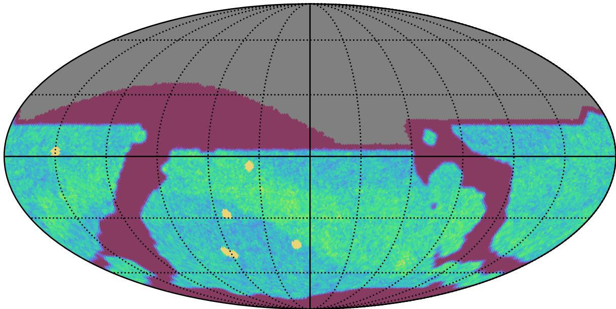
internal_u_expt38_nscale1.2v3.4_10yrs All sky i band: NVisits
