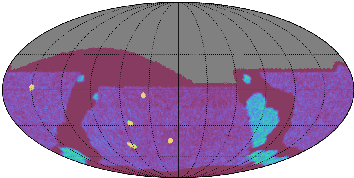
internal_u_expt38_nscale1.2v3.4_10yrs All sky g band: NVisits
