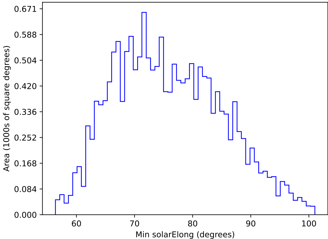
internal_u_expt38_nscale1.2v3.4_10yrs WFD u band: Min solarElong
