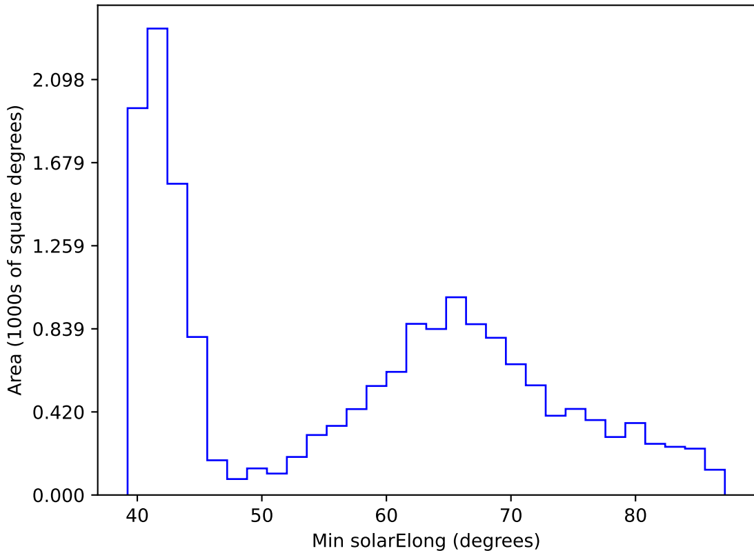
internal_u_expt38_nscale1.2v3.4_10yrs WFD r band: Min solarElong
