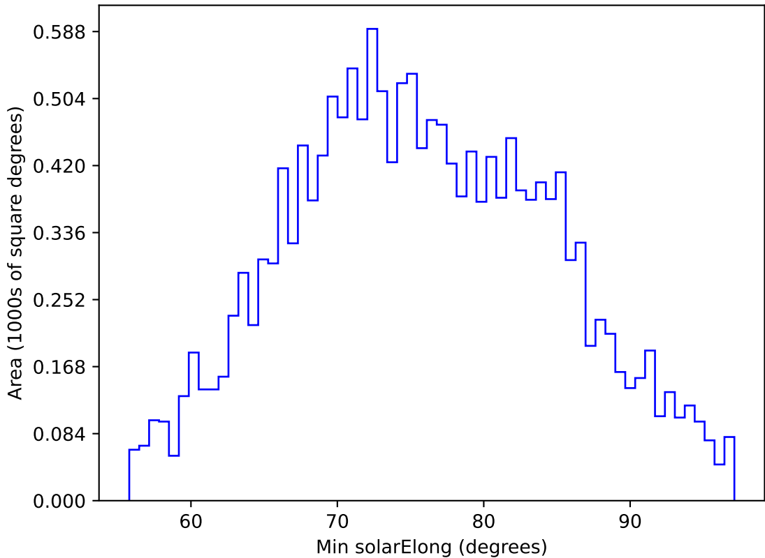
internal_u_expt38_nscale1.2v3.4_10yrs WFD g band: Min solarElong
