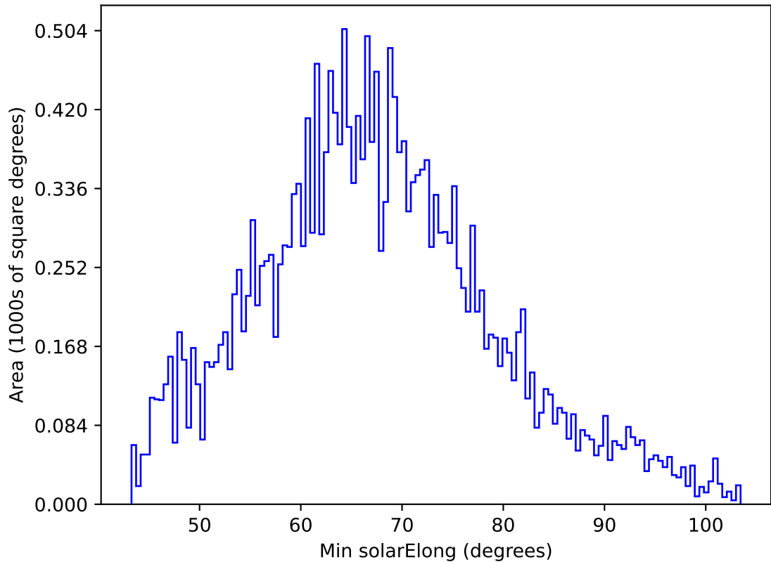
internal_u_expt38_nscale1.2v3.4_10yrs All sky y band: Min solarElong
