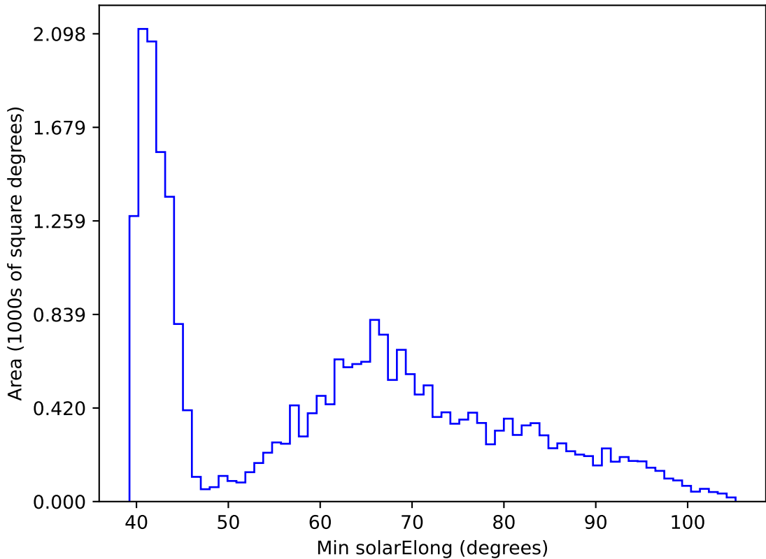
internal_u_expt38_nscale1.2v3.4_10yrs All sky r band: Min solarElong
