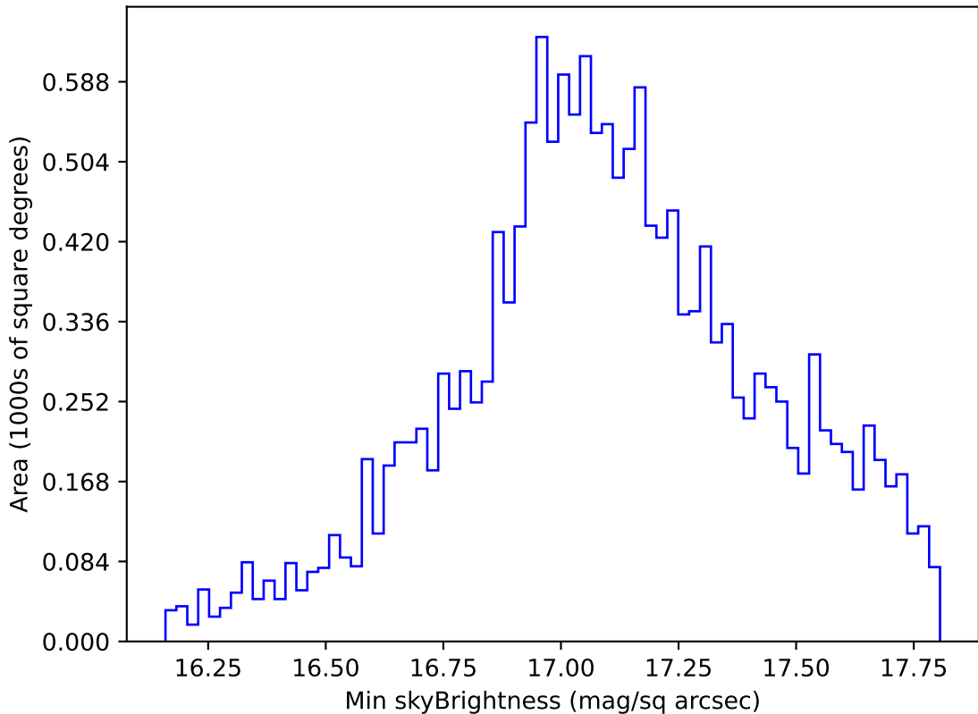
internal_u_expt38_nscale1.2v3.4_10yrs WFD y band: Min skyBrightness
