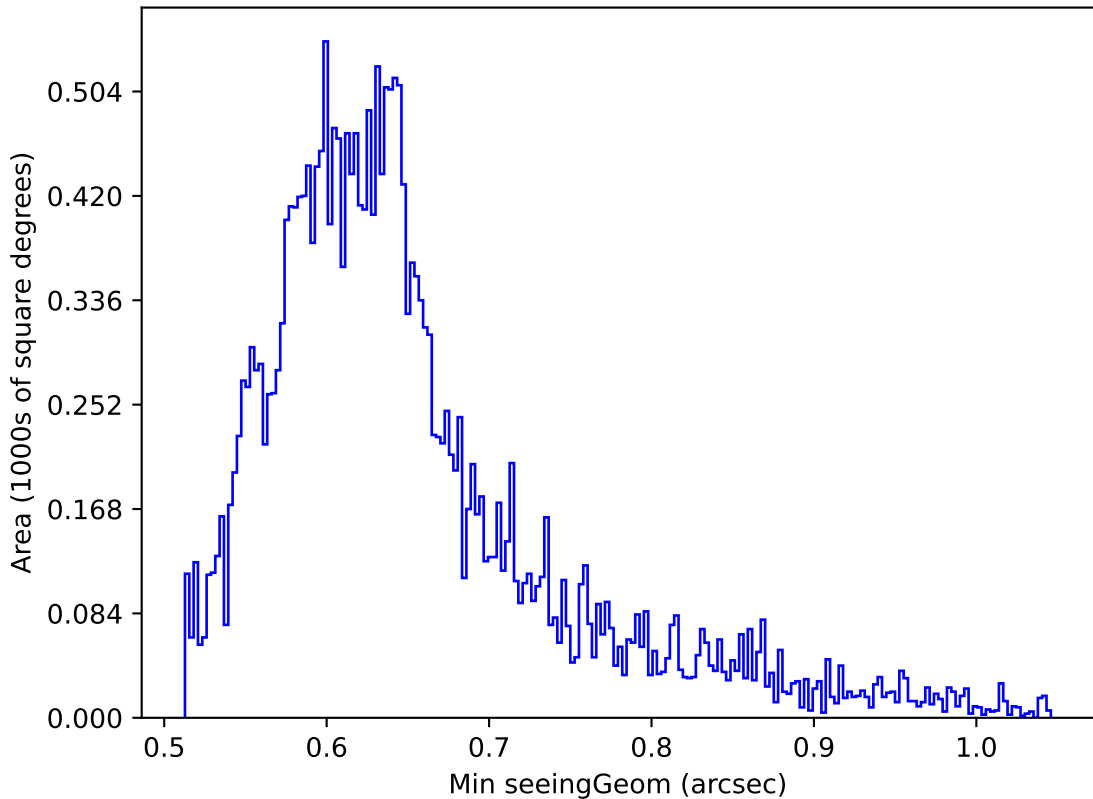
internal_u_expt38_nscale1.2v3.4_10yrs Yr 1 z band: Min seeingGeom
