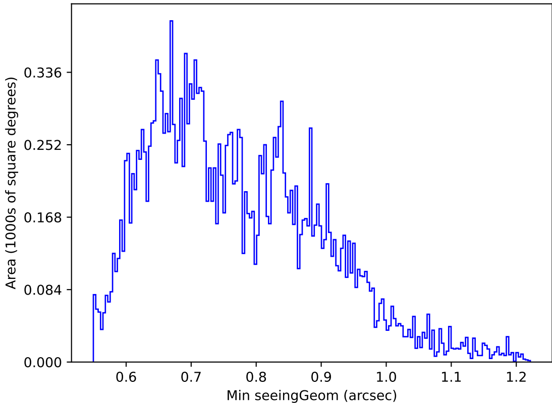
internal_u_expt38_nscale1.2v3.4_10yrs Yr 1 u band: Min seeingGeom
