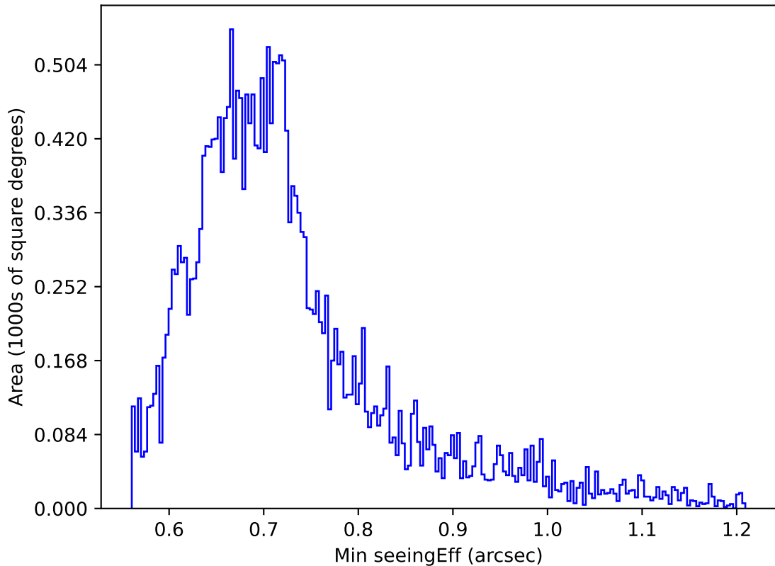
internal_u_expt38_nscale1.2v3.4_10yrs Yr 1 z band: Min seeingEff
