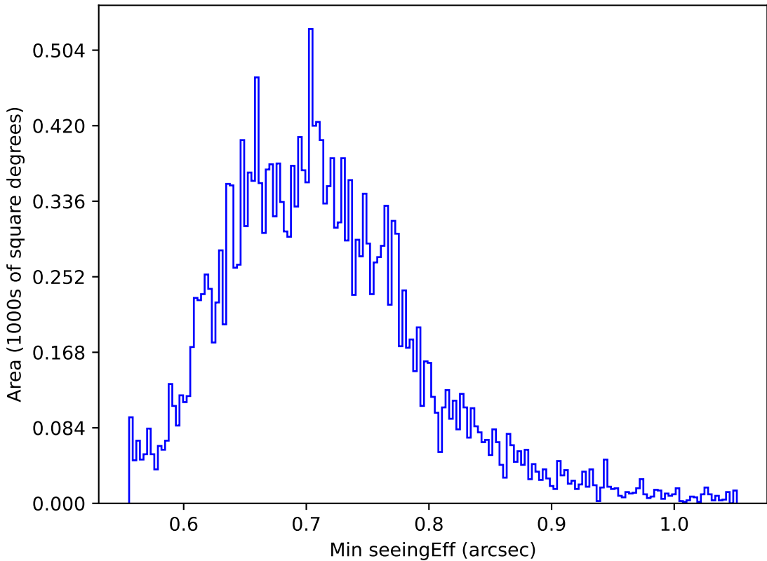
internal_u_expt38_nscale1.2v3.4_10yrs Yr 1 y band: Min seeingEff
