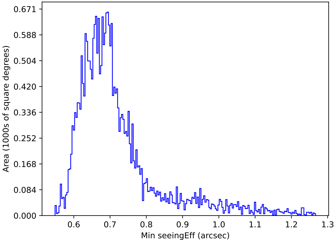
internal_u_expt38_nscale1.2v3.4_10yrs Yr 1 r band: Min seeingEff
