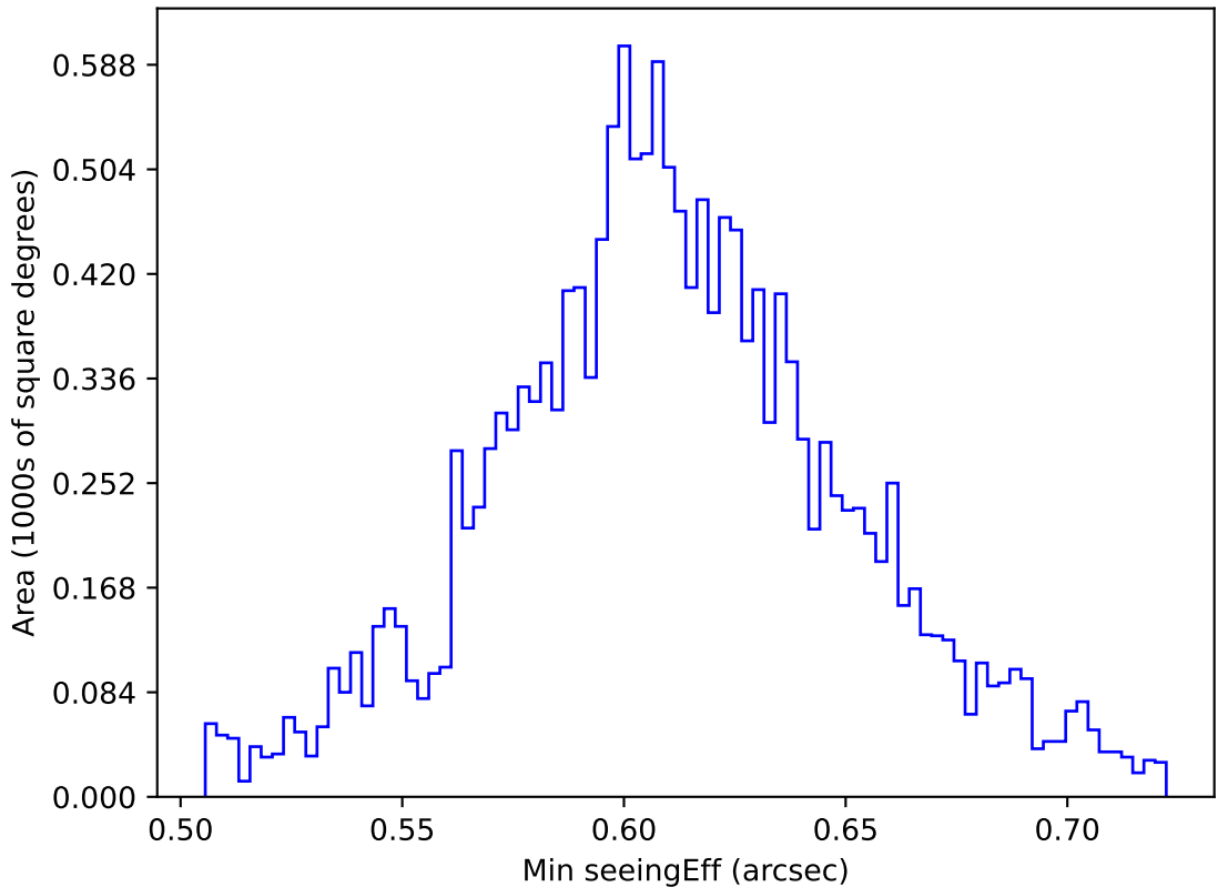
internal_u_expt38_nscale1.2v3.4_10yrs WFD z band: Min seeingEff
