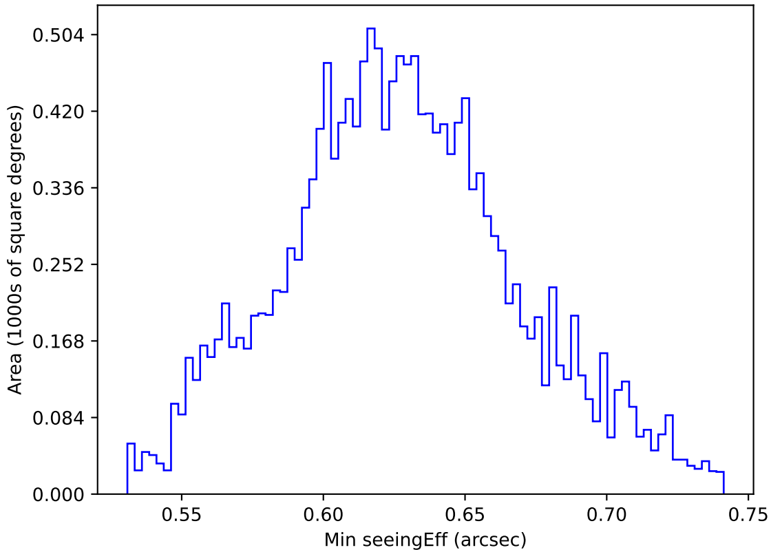
internal_u_expt38_nscale1.2v3.4_10yrs WFD y band: Min seeingEff
