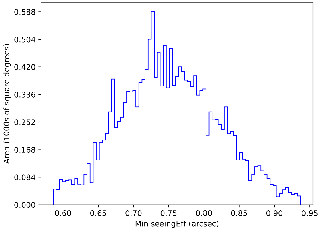
internal_u_expt38_nscale1.2v3.4_10yrs WFD u band: Min seeingEff
