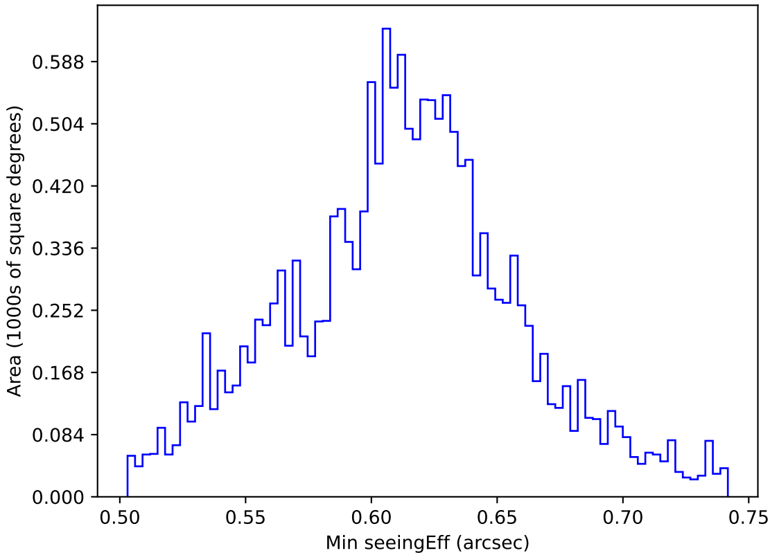
internal_u_expt38_nscale1.2v3.4_10yrs WFD r band: Min seeingEff
