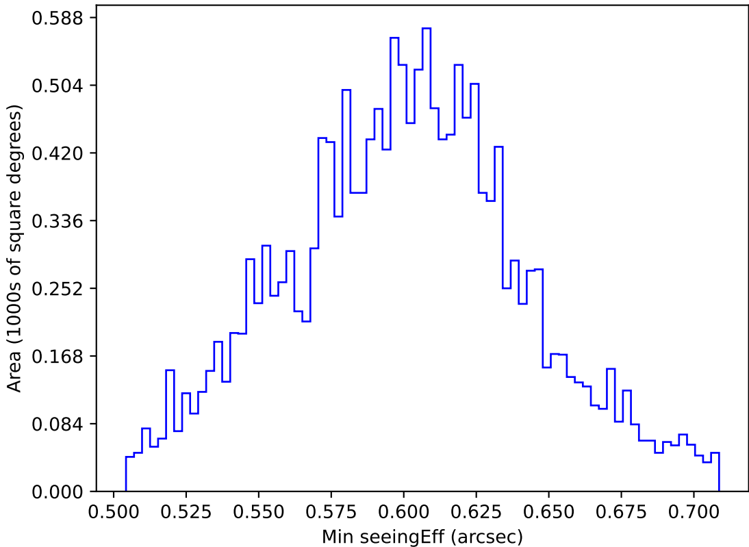
internal_u_expt38_nscale1.2v3.4_10yrs WFD i band: Min seeingEff
