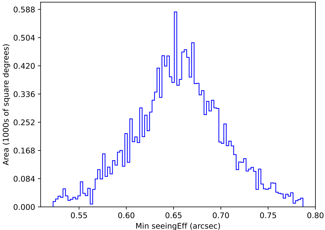
internal_u_expt38_nscale1.2v3.4_10yrs WFD g band: Min seeingEff
