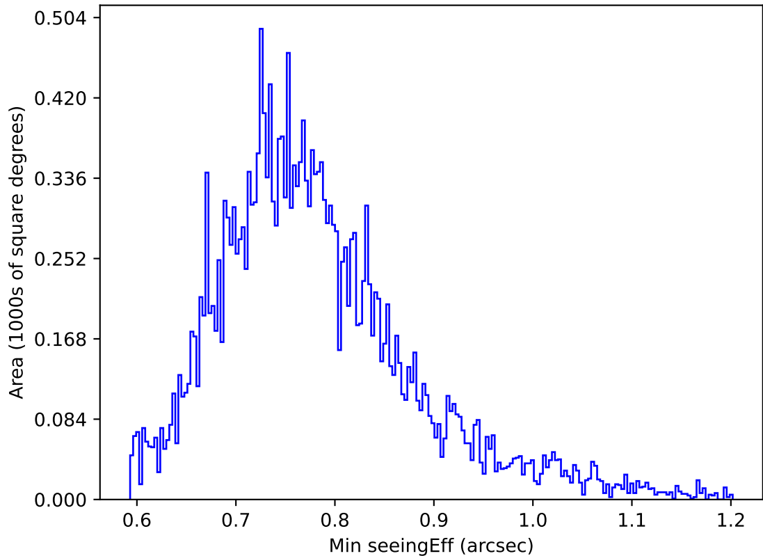
internal_u_expt38_nscale1.2v3.4_10yrs All sky u band: Min seeingEff
