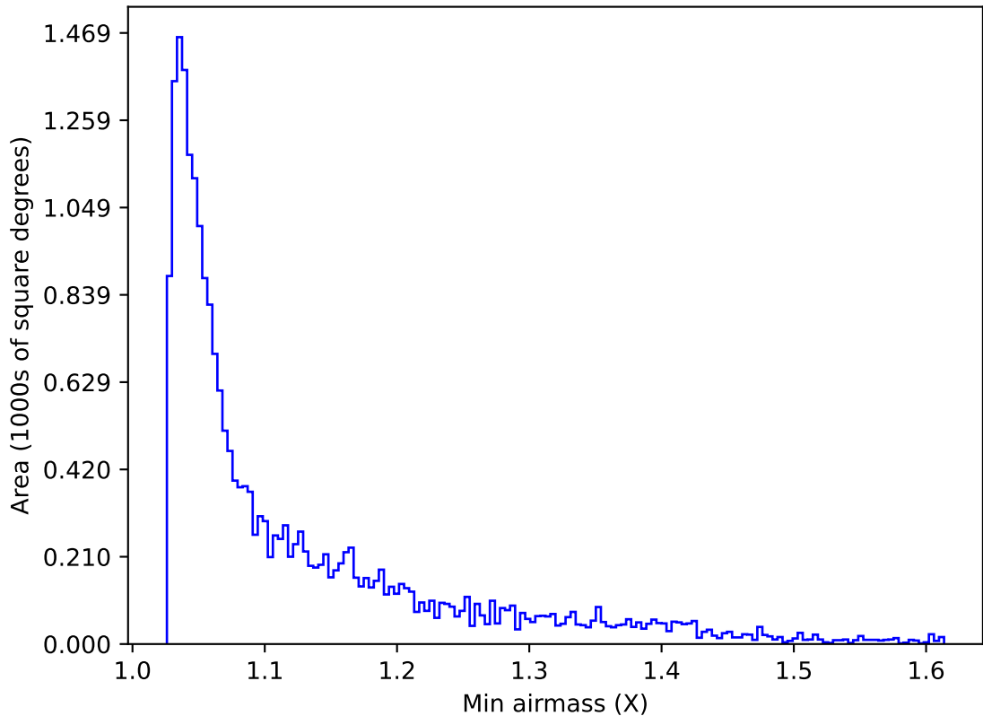
internal_u_expt38_nscale1.2v3.4_10yrs Yr 1 y band: Min airmass
