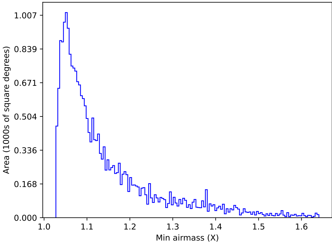
internal_u_expt38_nscale1.2v3.4_10yrs Yr 1 u band: Min airmass
