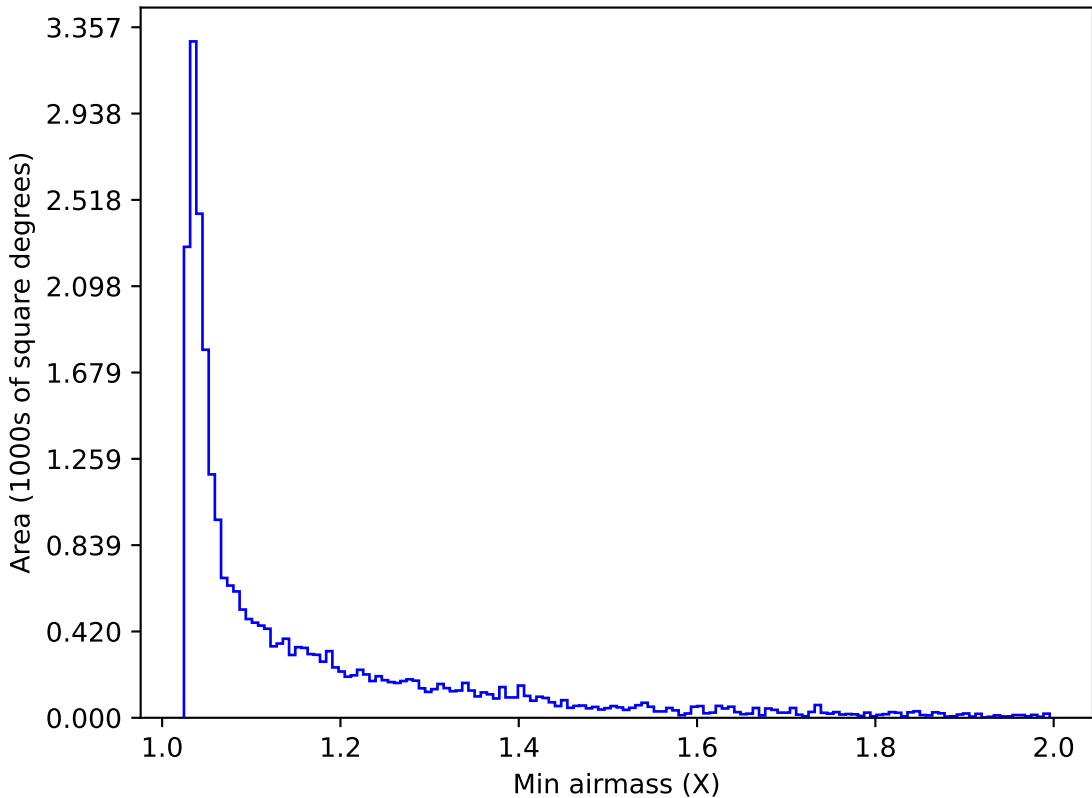
internal_u_expt38_nscale1.2v3.4_10yrs Yr 1 i band: Min airmass
