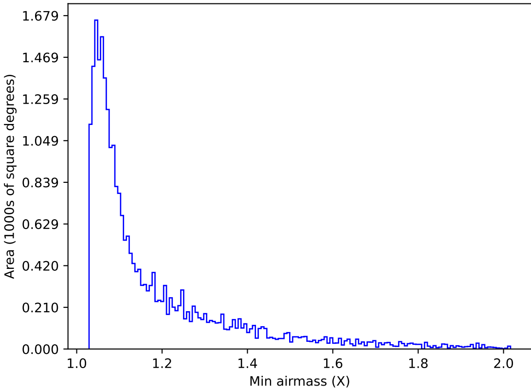
internal_u_expt38_nscale1.2v3.4_10yrs Yr 1 g band: Min airmass
