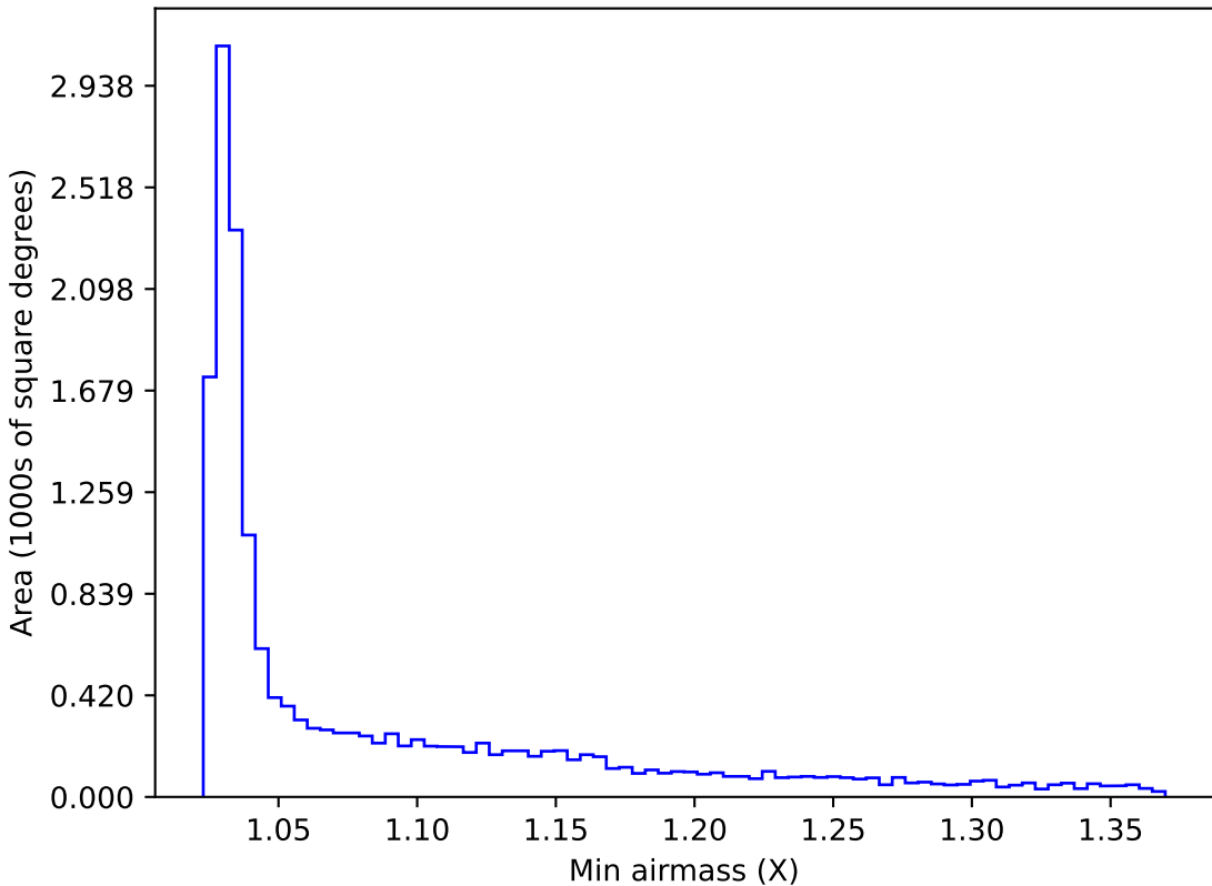
internal_u_expt38_nscale1.2v3.4_10yrs WFD y band: Min airmass
