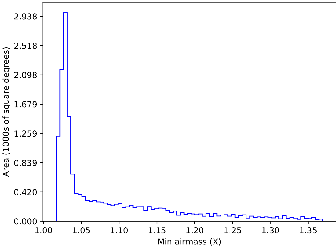
internal_u_expt38_nscale1.2v3.4_10yrs WFD r band: Min airmass
