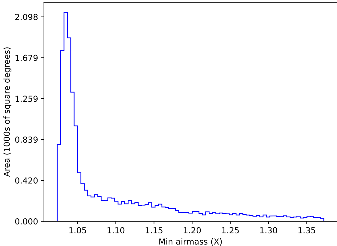
internal_u_expt38_nscale1.2v3.4_10yrs WFD g band: Min airmass
