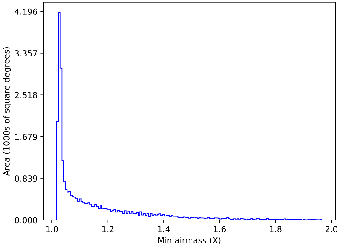
internal_u_expt38_nscale1.2v3.4_10yrs All sky r band: Min airmass
