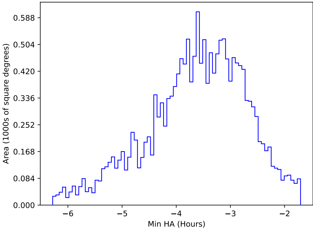
internal_u_expt38_nscale1.2v3.4_10yrs WFD y band: Min HA
