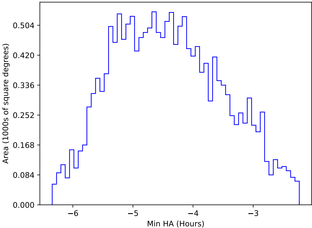
internal_u_expt38_nscale1.2v3.4_10yrs WFD r band: Min HA
