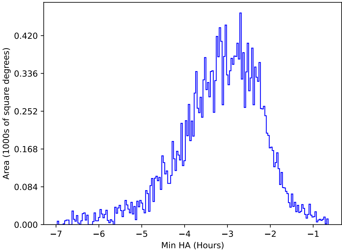
internal_u_expt38_nscale1.2v3.4_10yrs All sky u band: Min HA
