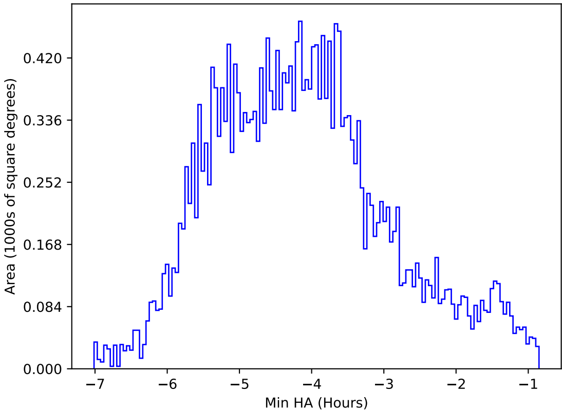
internal_u_expt38_nscale1.2v3.4_10yrs All sky r band: Min HA
