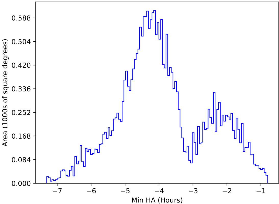
internal_u_expt38_nscale1.2v3.4_10yrs All sky g band: Min HA
