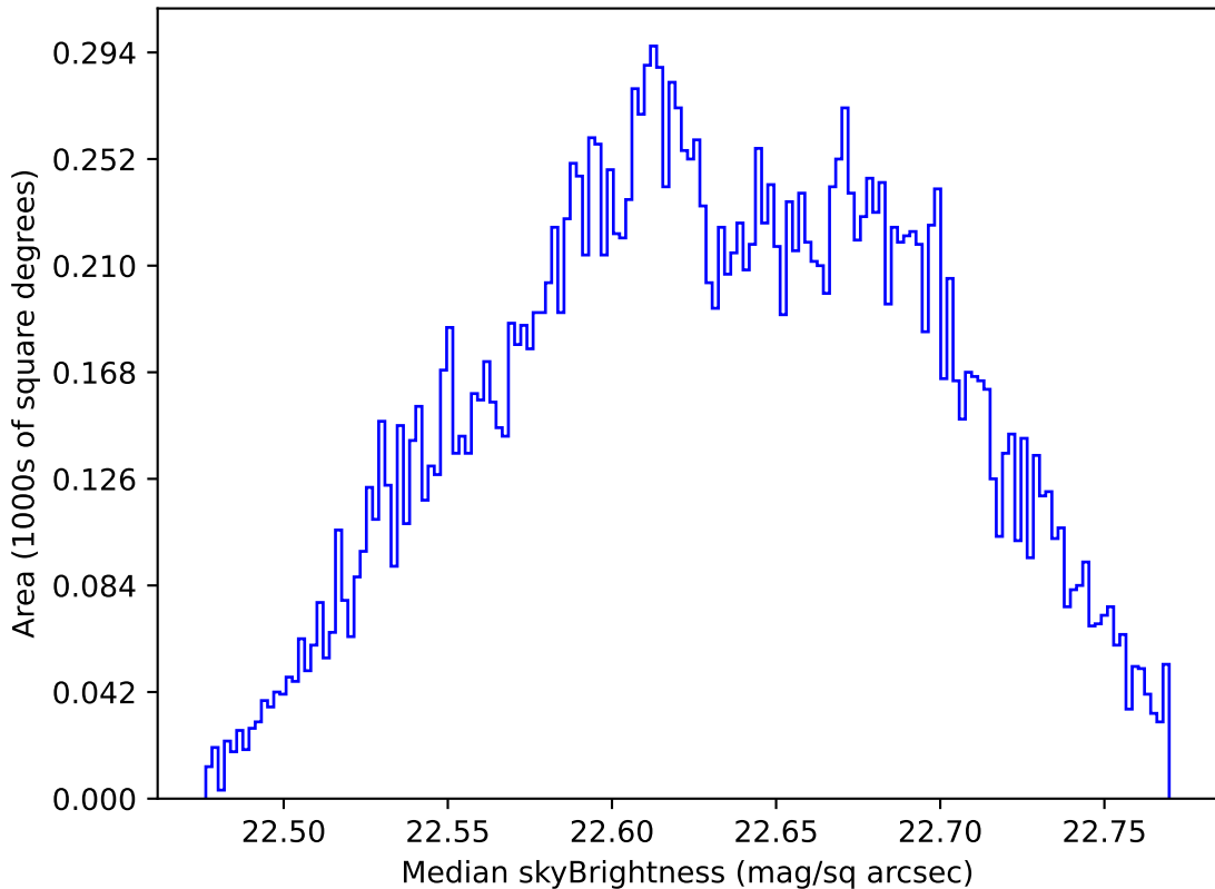
internal_u_expt38_nscale1.2v3.4_10yrs Yr 1 u band: Median skyBrightness
