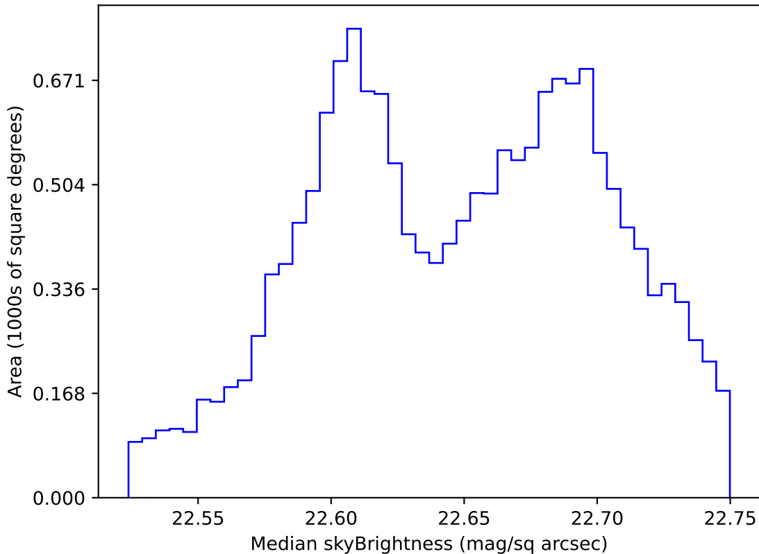
internal_u_expt38_nscale1.2v3.4_10yrs WFD u band: Median skyBrightness
