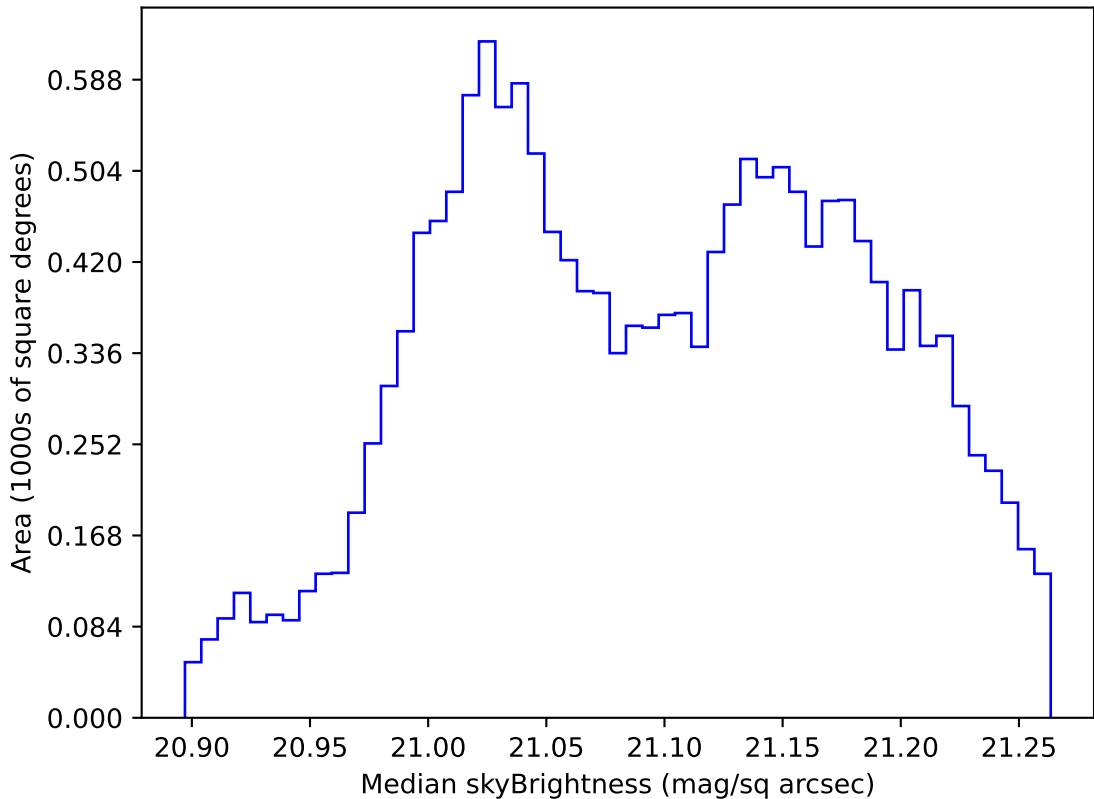
internal_u_expt38_nscale1.2v3.4_10yrs WFD r band: Median skyBrightness
