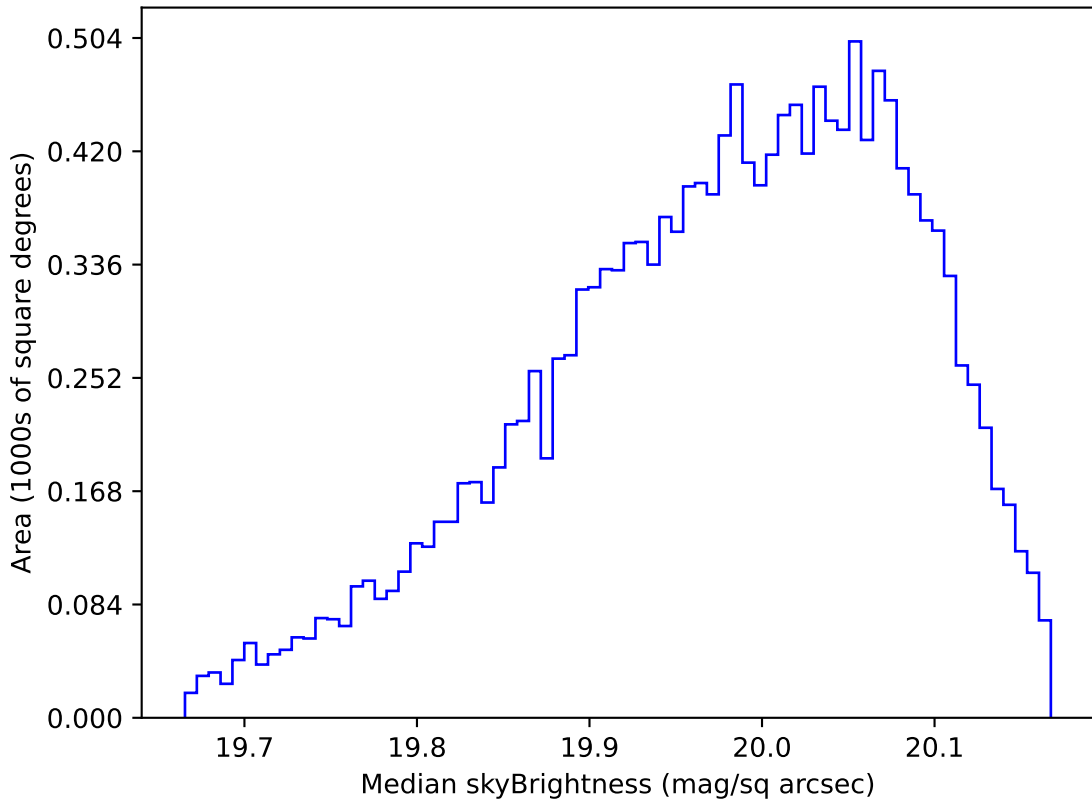
internal_u_expt38_nscale1.2v3.4_10yrs WFD i band: Median skyBrightness
