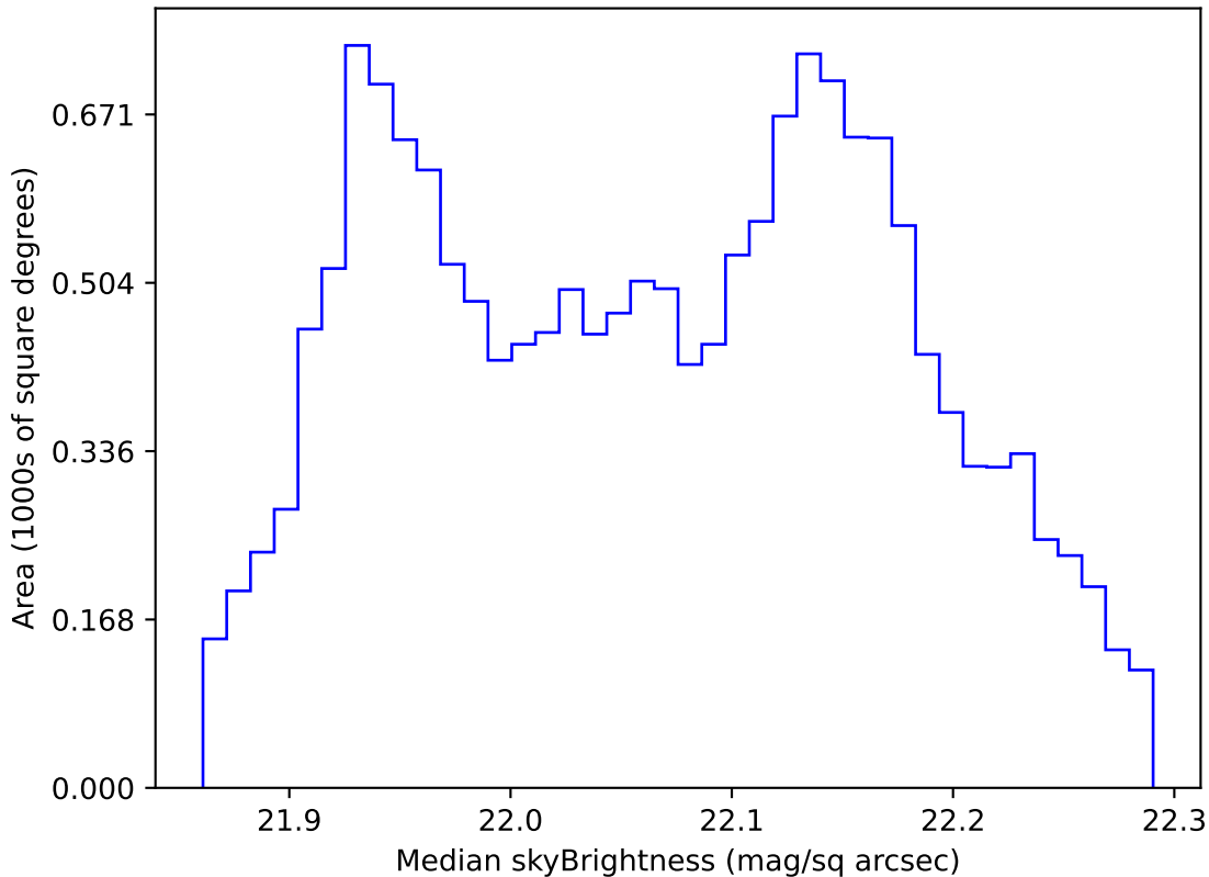
internal_u_expt38_nscale1.2v3.4_10yrs WFD g band: Median skyBrightness
