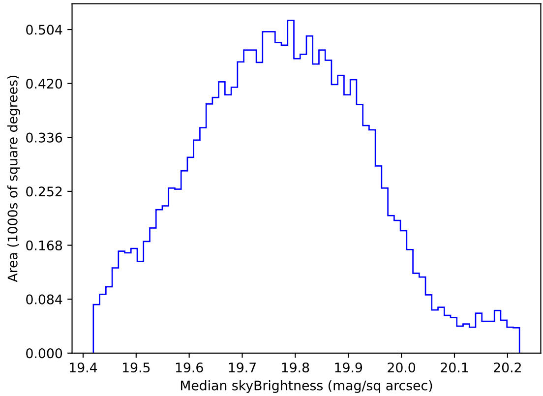
internal_u_expt38_nscale1.2v3.4_10yrs WFD all bands: Median skyBrightness
