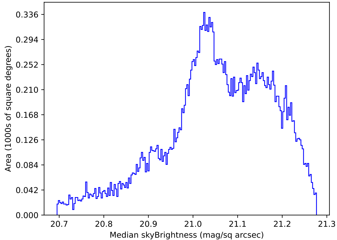
internal_u_expt38_nscale1.2v3.4_10yrs All sky r band: Median skyBrightness
