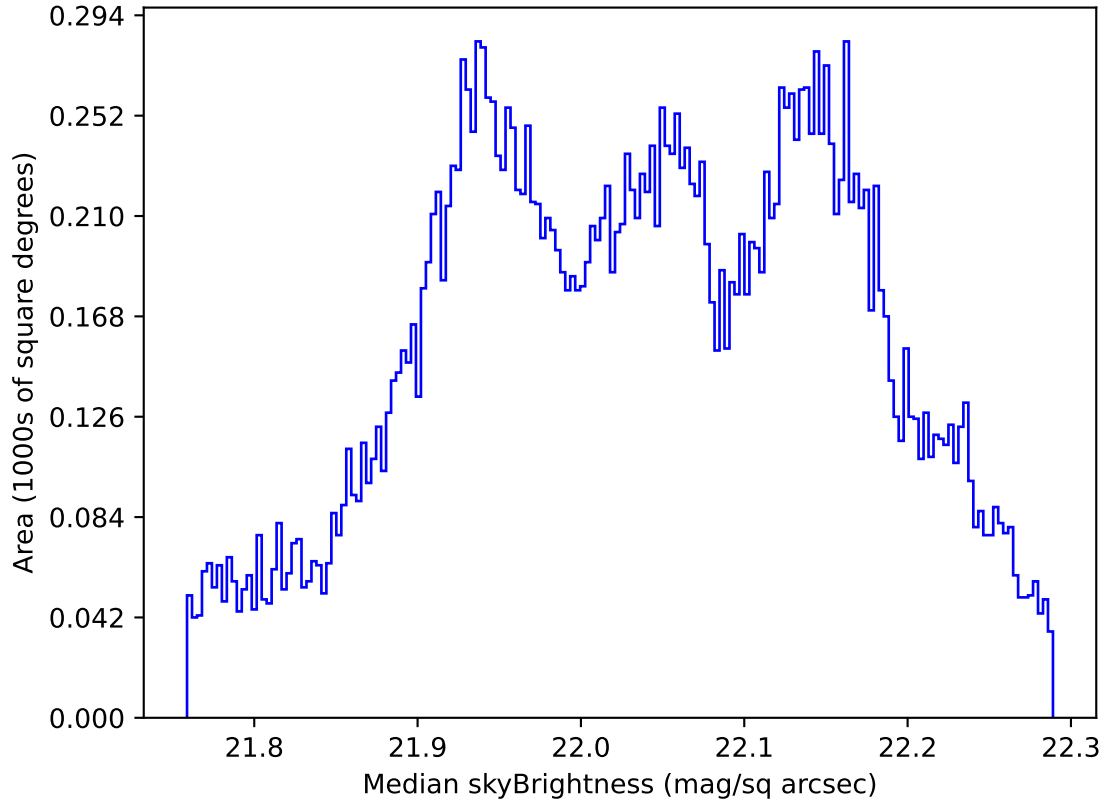
internal_u_expt38_nscale1.2v3.4_10yrs All sky g band: Median skyBrightness
