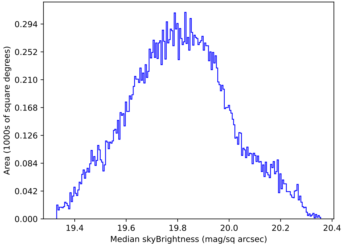
internal_u_expt38_nscale1.2v3.4_10yrs All sky all bands: Median skyBrightness
