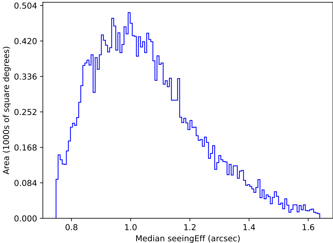
internal_u_expt38_nscale1.2v3.4_10yrs Yr 1 g band: Median seeingEff
